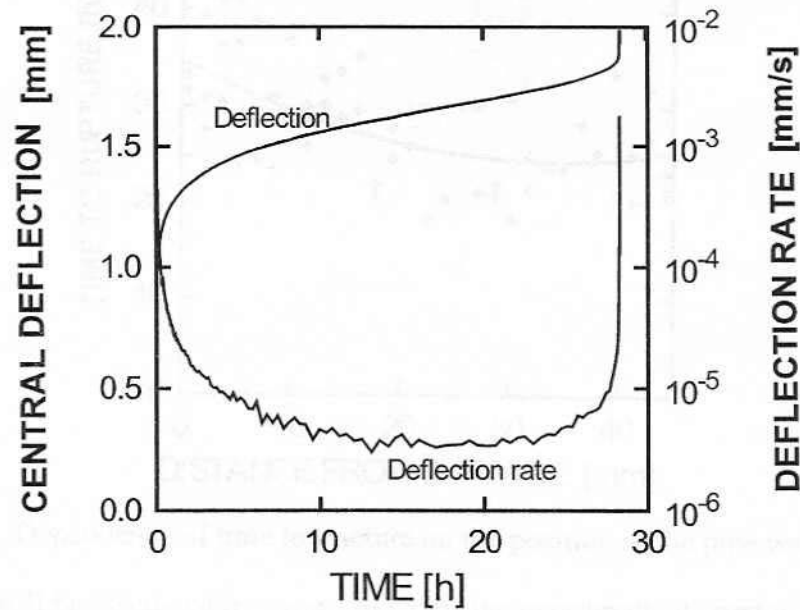
Fig. A3.3: The deflection versus time and deflection rate versus time curve of small sample creep test
