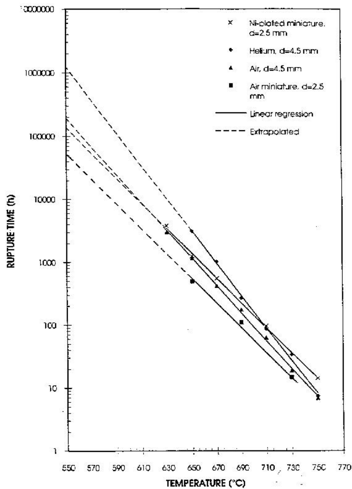
Figure A1.3: Efficiency of oxidation protection methods for microspecimen testing [1]
