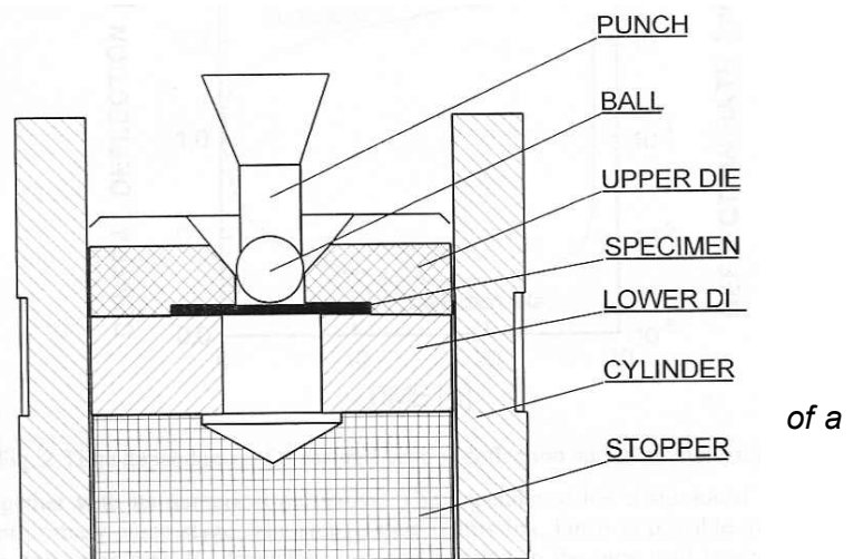
Fig A3.1: Schematic sketch small punch bulge test
