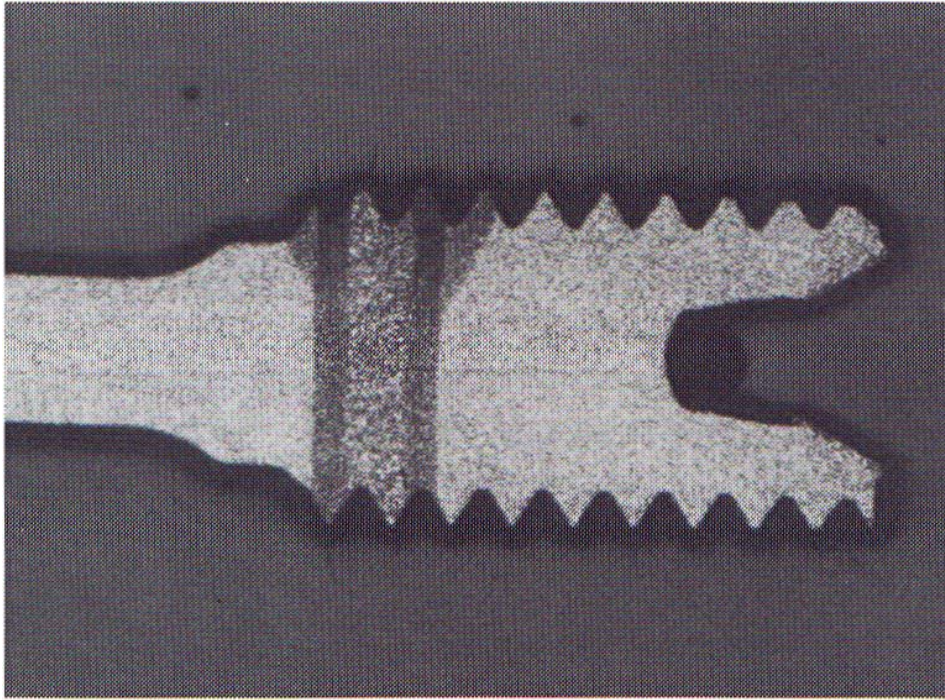
Figure 5. The electron beam welded creep specimen where the weldment lies inside the threaded ends (Ref. 7).
