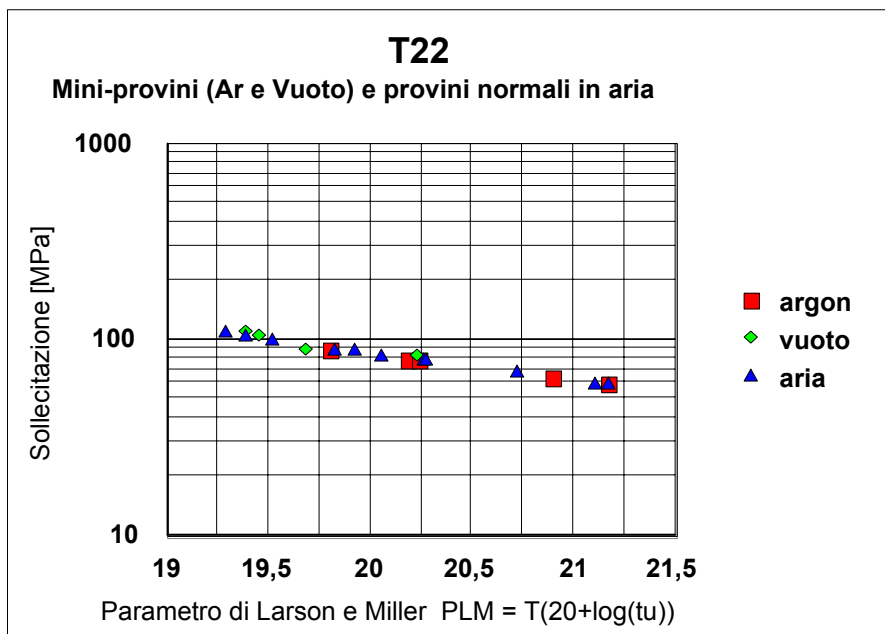
Figure A1.2: Comparison of Larson-Miller parametrised creep rupture strength of virgin 2,25Cr-1Mo conventional specimens tested in air (triangles), microspecimens tested in Argon (squares) and in vacuum (rhombi) [3]
