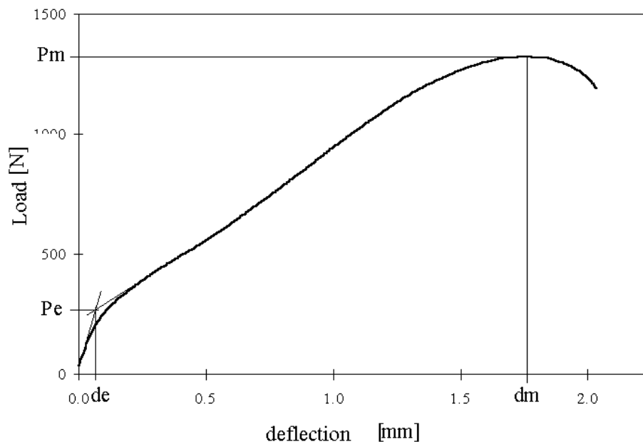
Fig. A3.2: Load-deflection curve of a small punch test
