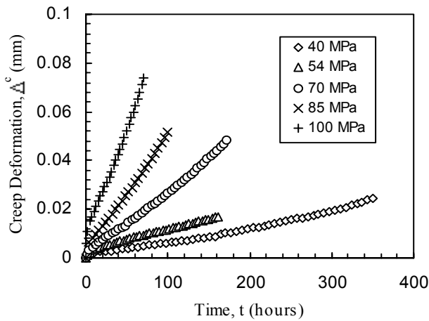
Fig.A2.2 Creep deformation from impression creep tests for the HAZ material in a 2-
