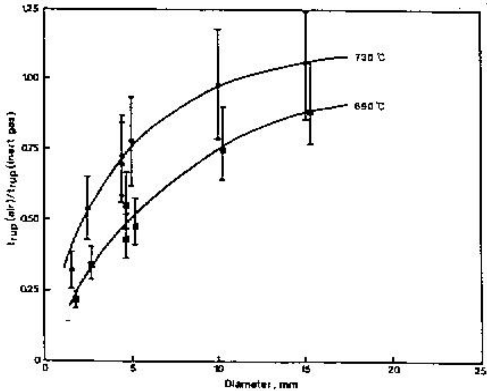
Figure A1.1: Effect of oxidation on creep rupture time depending on specimen diameter [1]
